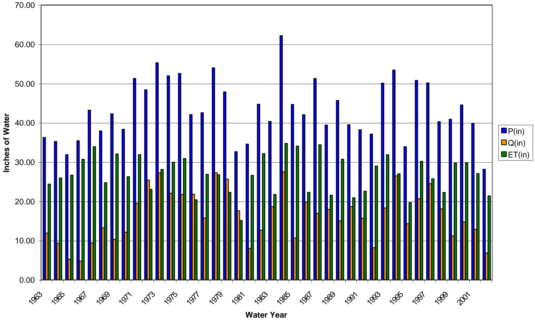
Annual Water Budget for Monocacy Creek 1963-2002
